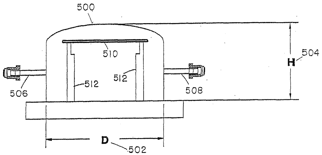
Wafer Chamber
